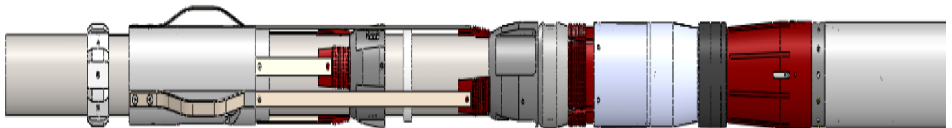
Allamon Liner Hanger tool
